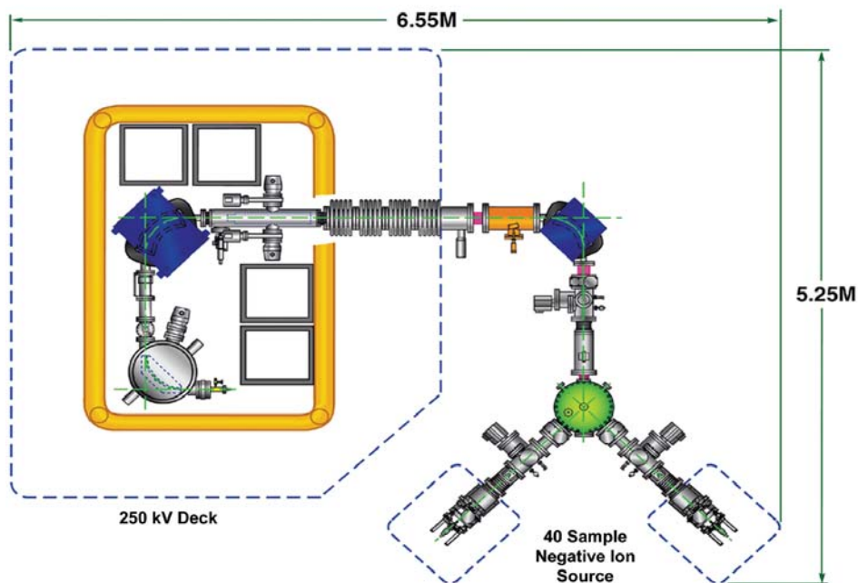
Figure 3: The first commercial Single Stage AMS system is equipped with a sequential injection, dual ion source injector allowing mass 12 and 13 to be measured after the final 90° analyzing magnet. This configuration is the reverse of the prototype with the injector system at ground to allow greater sample handling flexibility.
