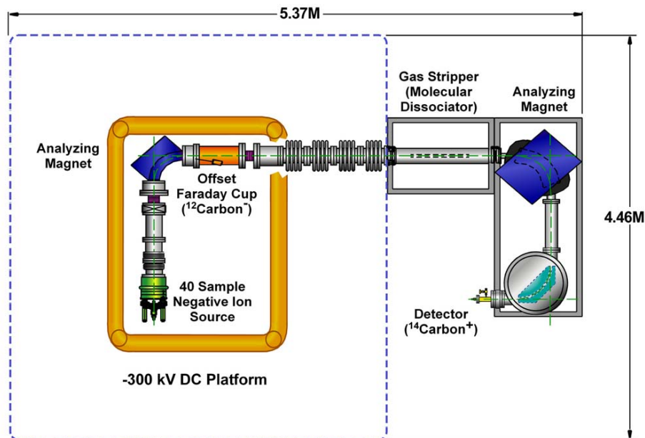
Figure 2: The prototype Single Stage AMS system has the 40 sample negative carbon source followed by a 90° permanent magnet for mass analysis. Only the mass 12 beam was measured before acceleration. The gas stripper, 90° analyzing magnet, 90° electrostatic spherical analyzer and detector are located at ground potential.
