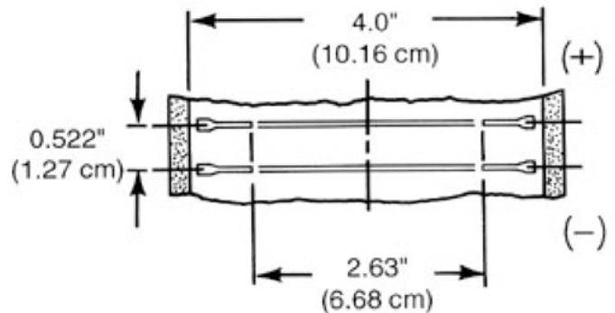
Cross-sectional view showing detachable internal electrodes of the high gradient acceleration tube section
