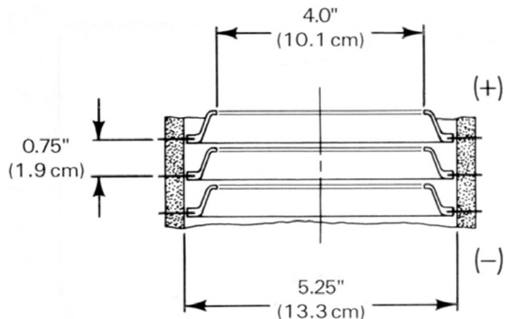
Cross-sectional view showing detachable internal electrodes of the general purpose acceleration tube section. Dimensions vary slightly for non-magnetic model
