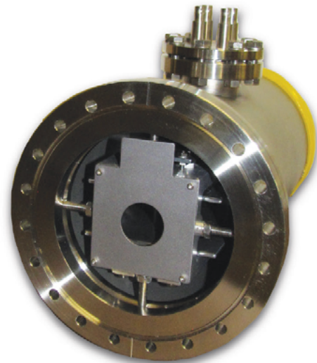
Electrostatic X-Y ion beam steerer with NEC flanges. Entrance aperture visible.
