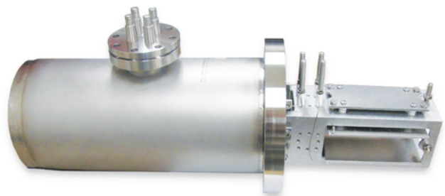
Inner assembly exposed. All plates assembled as one unit.
